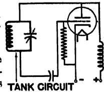
TANK CIRCUIT Ultraudion oscillator.
